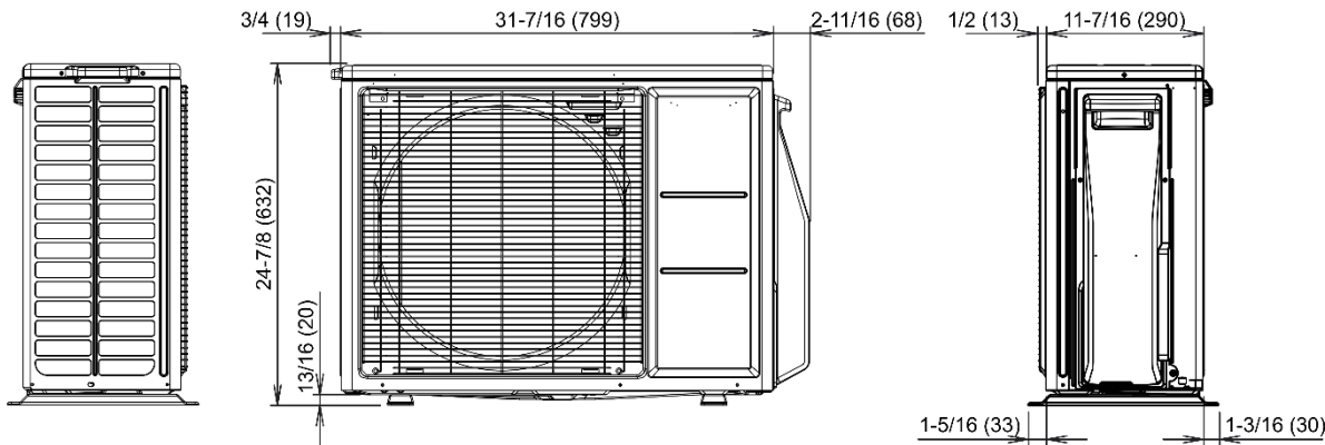
Side view
