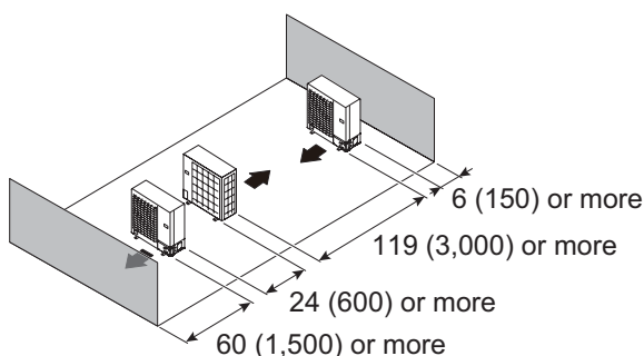
Single parallel unit arrangement
