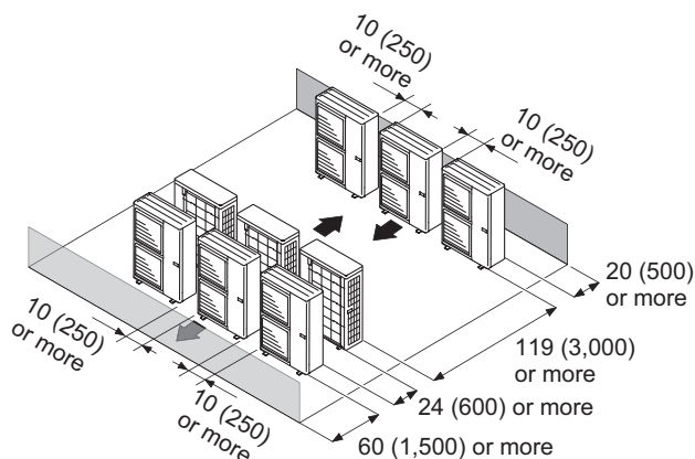
Multiple parallel unit arrangement
