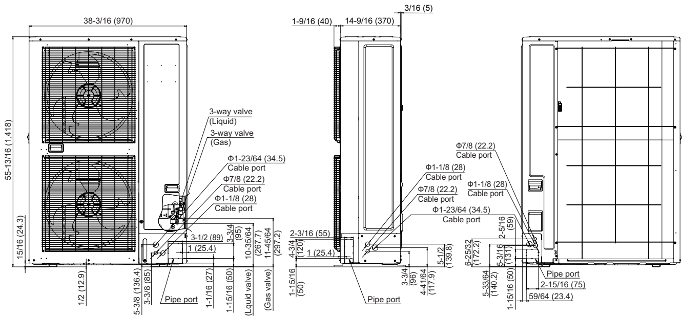
Front view
