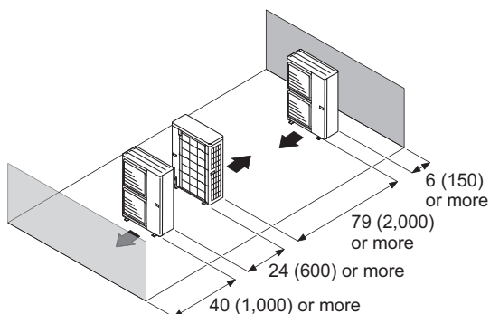
Single parallel unit arrangement
