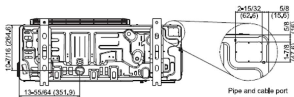
Bottom view
